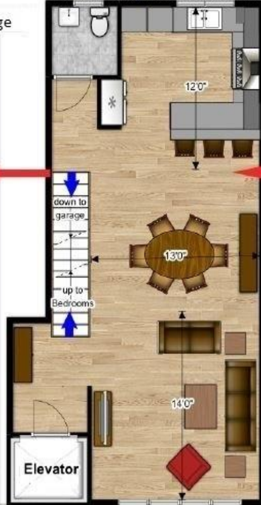
Second floor living/dining/kitchen/half bath
